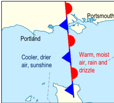
Air Mass Boundary
