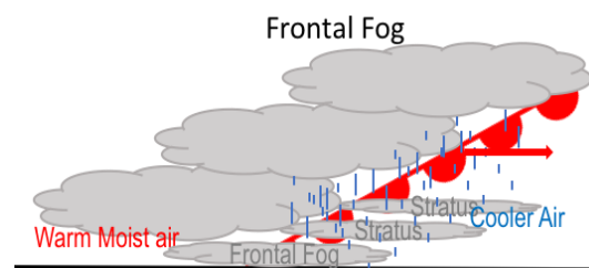
A Simple Depiction of Frontal Fog
